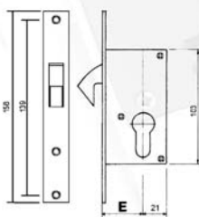
Hook bolt for Sliding Door
