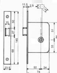
Latch only for Passage
