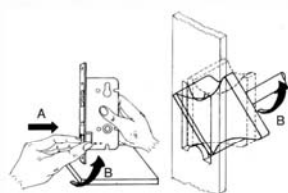
Reversible Latch
