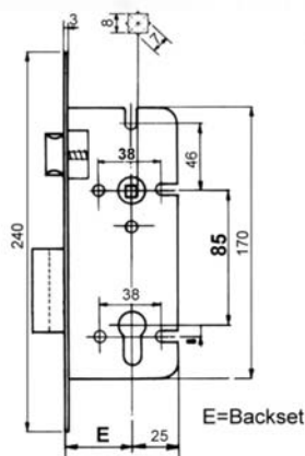
Art. 4510 E = 40 / 50mm
